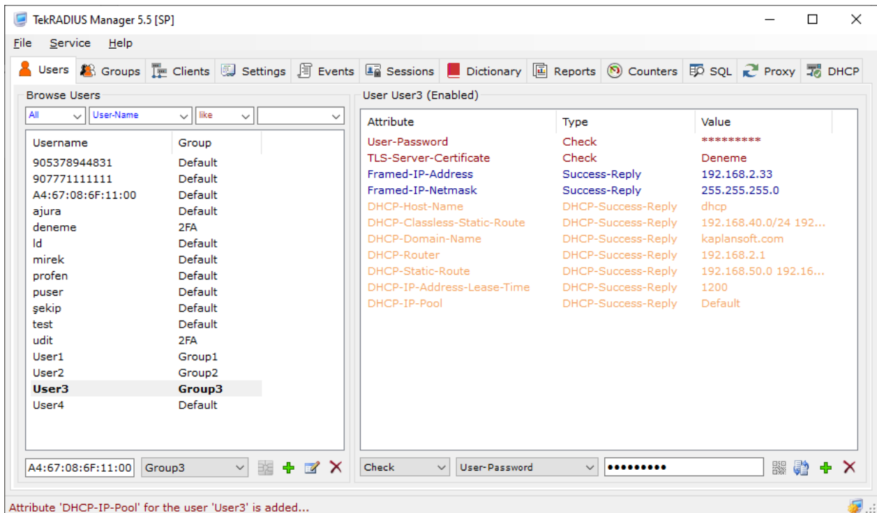
Figure 17 - User Profile with DHCP Options
