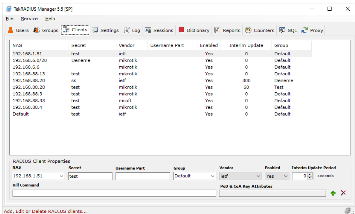
Figure 9 - RADIUS Clients
