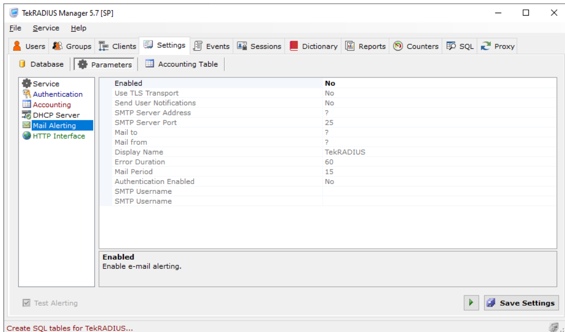
Figure 8 - Alerting Configuration
