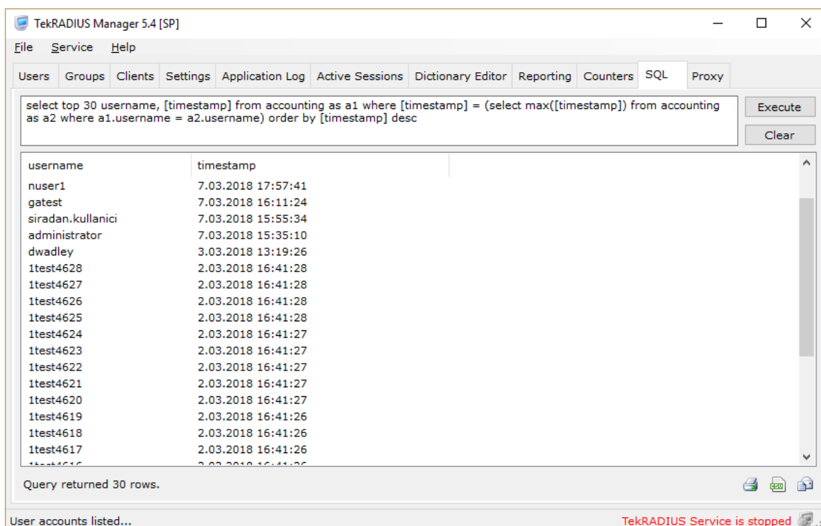
Figure 13 - SQL Query Executioner
