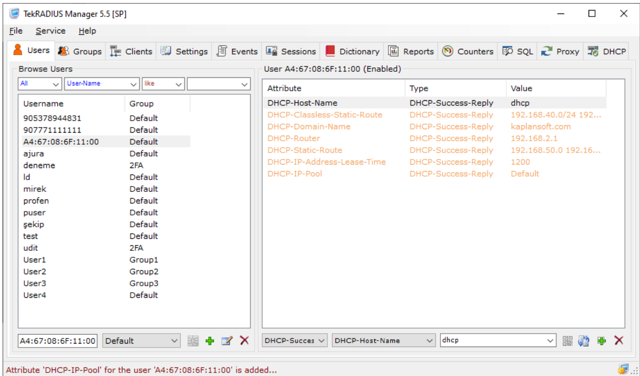
Figure 16 - DHCP Profile based on MAC Address
