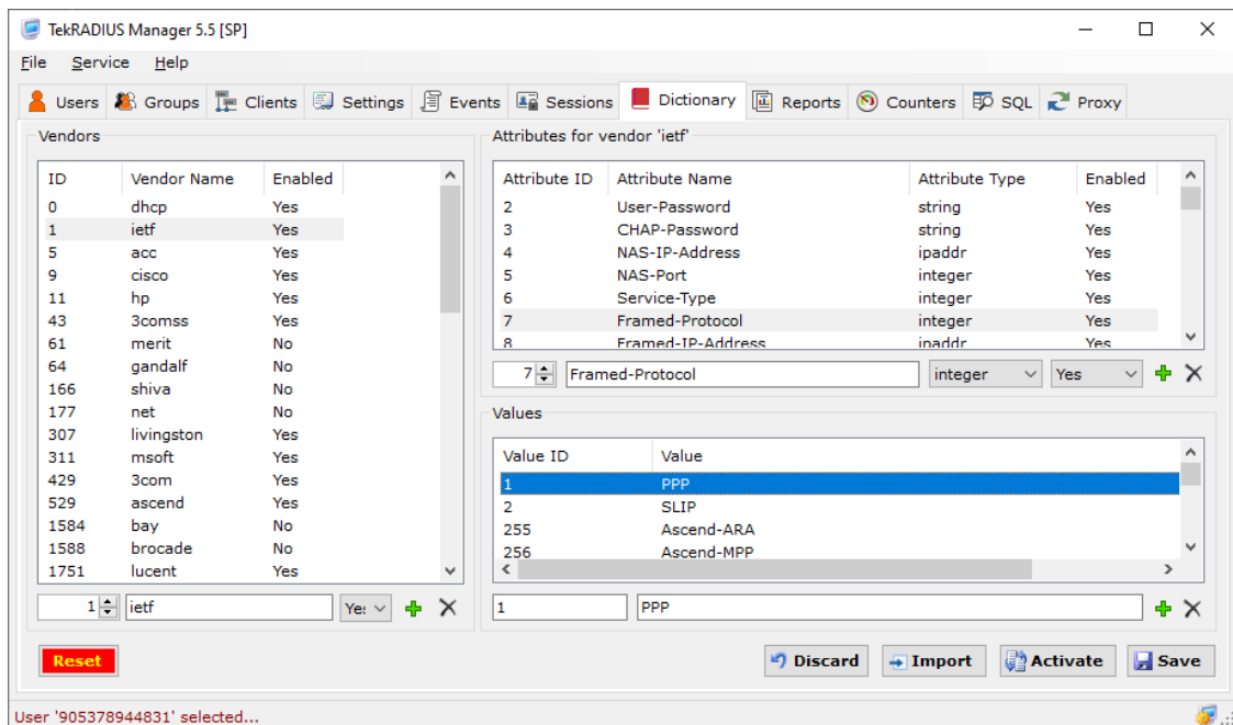
Figure 12 - Dictionary Editor
