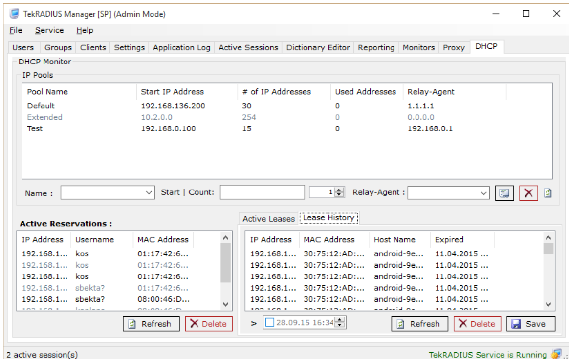
Figure 15 - DHCP Tab
