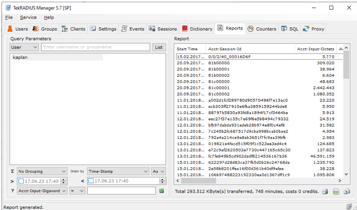
Figure 14 - Reporting Tab
