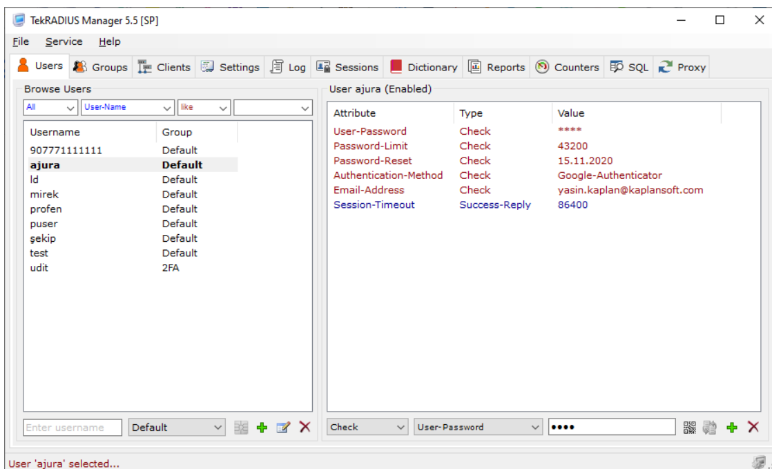
Figure 11 - Users Tab
