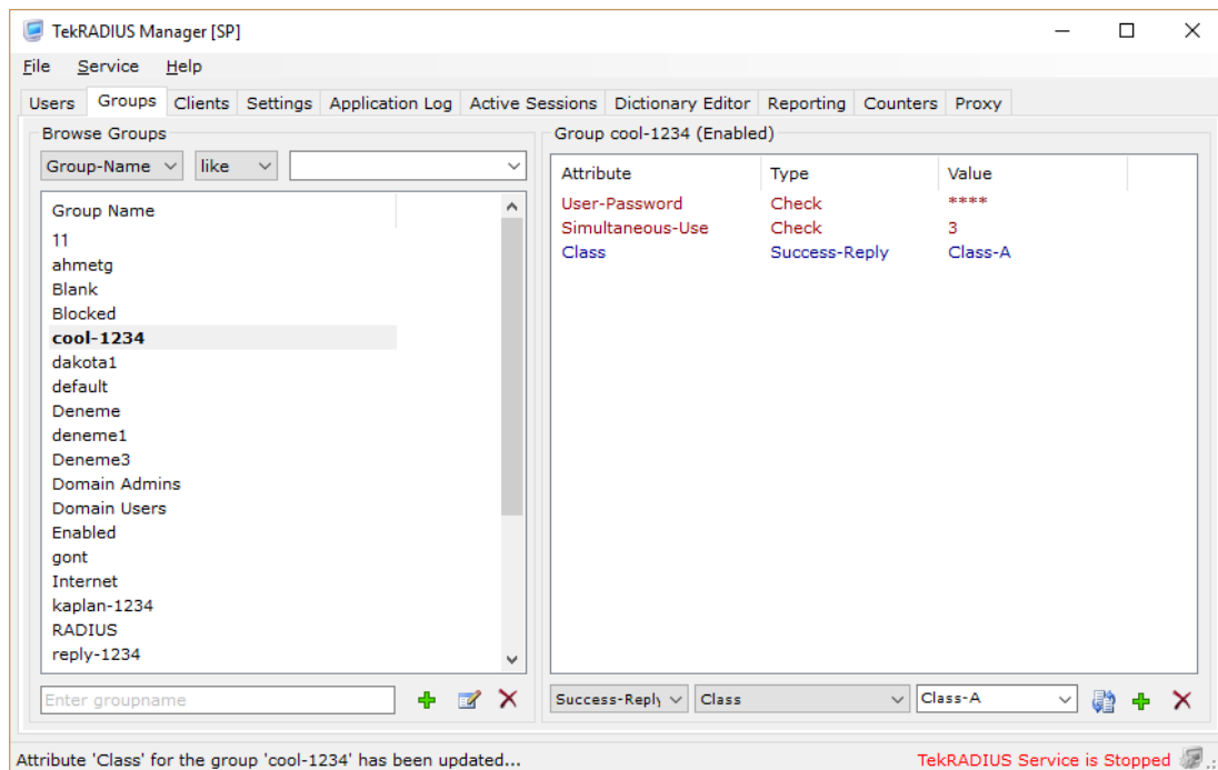
Figure 10 - Groups Tab
