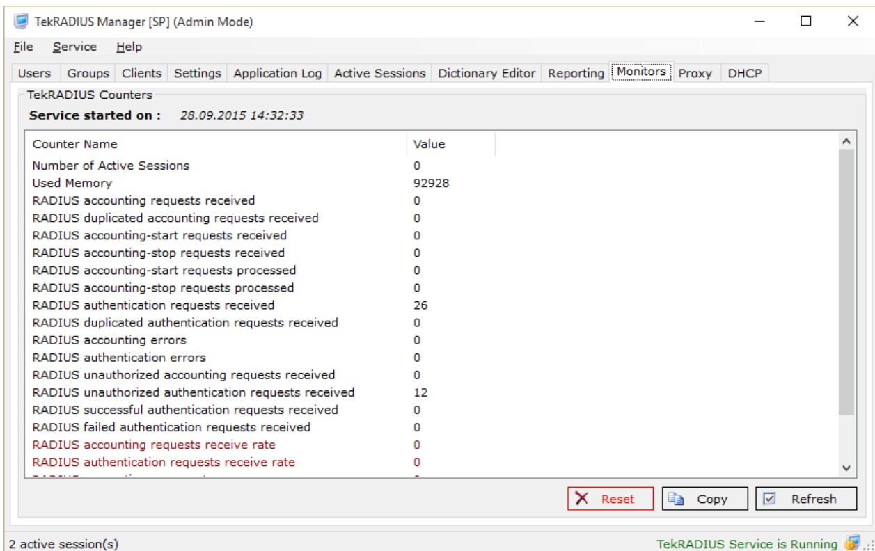
Figure 26. - TekRADIUS Manager Counters Tab
